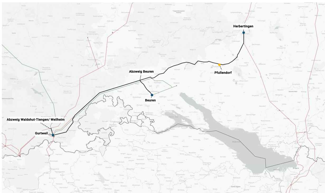
Map view TNG-P206
