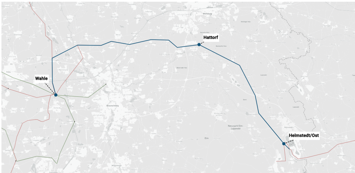
Map view TTG-P33
